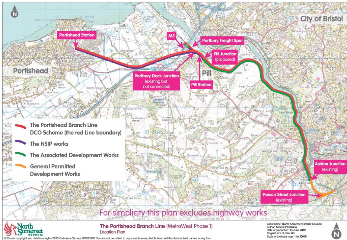
Figure 4.1: Location Plan
